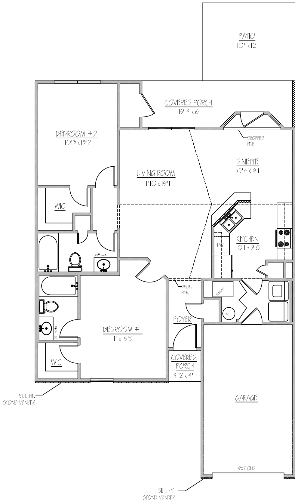
FLOOR PLAN ON SLAB
