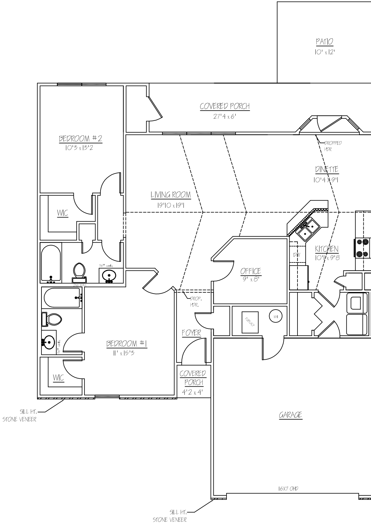
FLOOR PLAN ON SLAB
