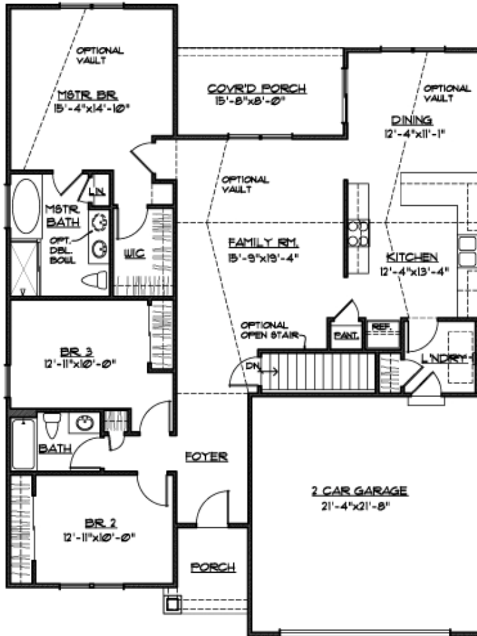
FIRST FLOOR PLAN W/ BASEMENT 3 BEDROOM
