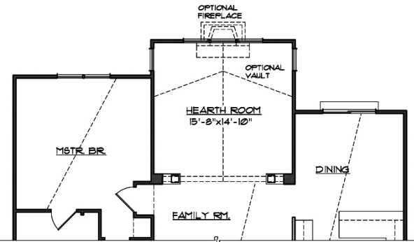
OPTIONAL HEARTH ROOM 3 BEDROOM
